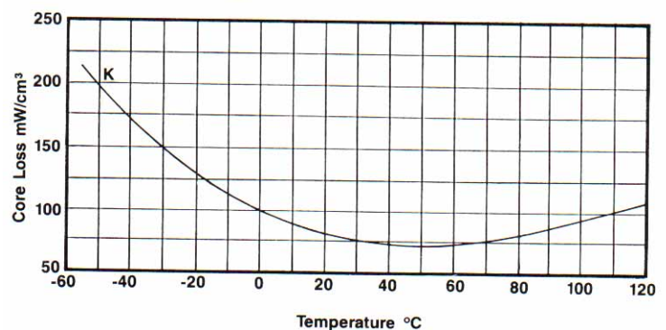
Figure 2 Core Loss vs. Temperature @ 500 kHz, 500 Gauss
